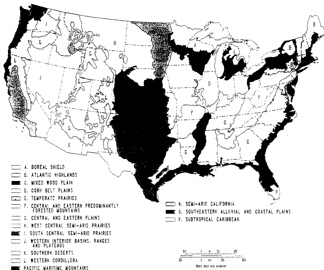
Figure 6. Omernik ecoregions and USGS hydrologic units.
