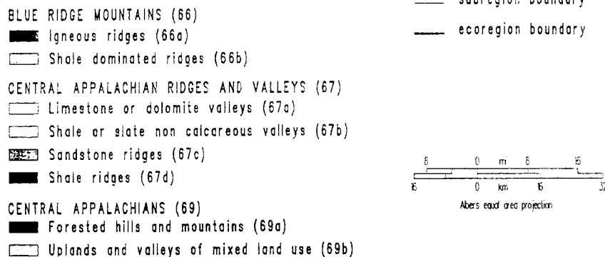
Figure 5. A portion of the ecoregions and subregions of EPA Region 3.
