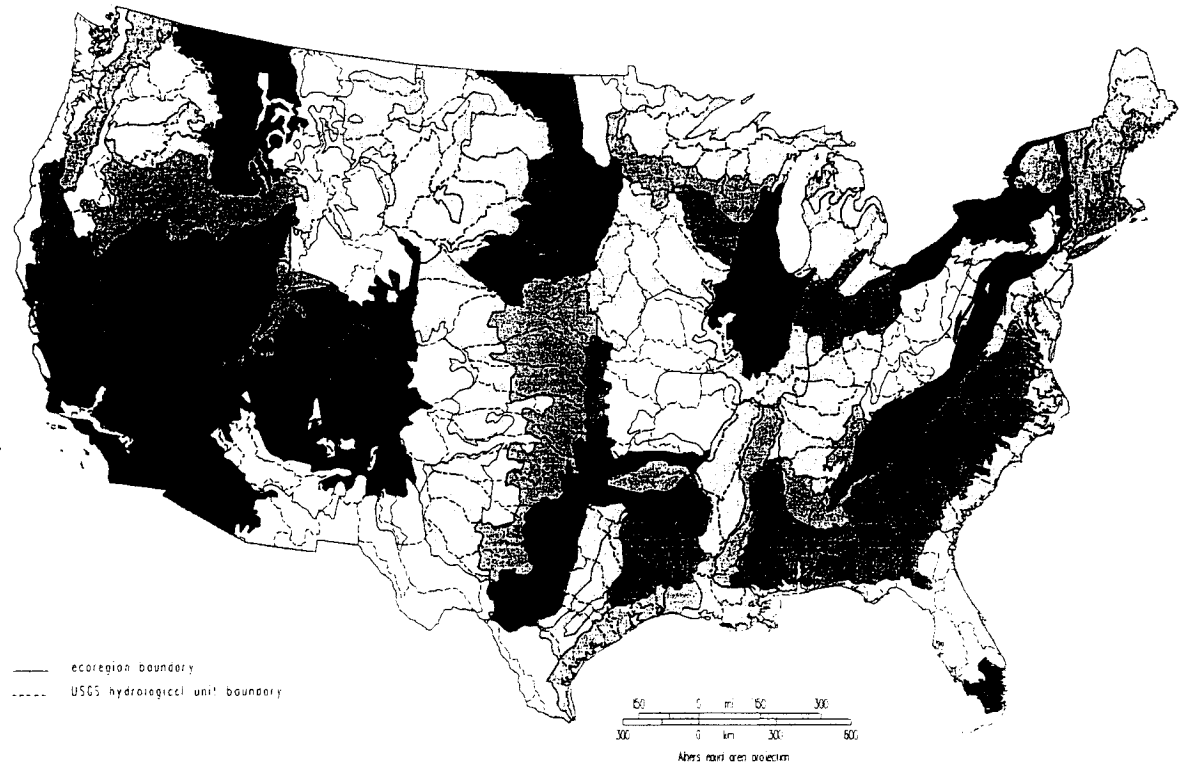
Figure 3. Ecological areas of the conterminous United States. (Adapted from Omernik, J. M. and Gallani, Proc. Global Nat. Resource Symp: Preparing for the 21st Century, Vol. 2, p. 943, 1990.)
