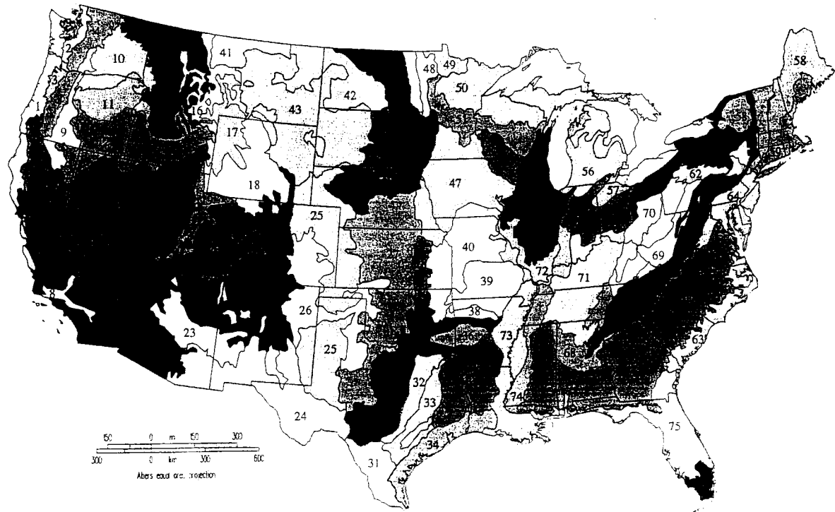
Figure 2. Ecoregions of the conterminous United States. 1 Coast Range, 2 Puget Lowland, 3 Willamette Valley, 4 Cascades, 5 Sierra Nevada, 6 Southern and Central California Plains and Hills, 7 Central California Valley, 8 Southern California Mountains, 9 Eastern Cascades Slopes and Foothills, 10 Columbia Plateau, 11 Blue Mountains, 12 Snake River Basin/High Desert, 13 Northern Basin and Range, 14 Southern Basin and Range, 15 Northern Rockies, 16 Montana Valley and Foothill Prairies, 17 Middle Rockies, 18 Wyoming Basin, 19 Wasatch and Uinta Mountains, 20 Colorado Plateaus, 21 Southern Rockies, 22 Arizona/New Mexico Plateau, 23 Arizona/New Mexico Mountains, 24 Southern Deserts, 25 Western High Plains, 26 Southwestern Tablelands, 27 Central Great Plains, 28 Flint Hills, 29 Central Oklahoma/Texas Plains, 30 Edwards Plateau, 31 Southern Texas Plains, 32 Texas Blackland Prairies, 33 East Central Texas Plains, 34 Western Gulf Coastal Plain, 35 South Central Plains, 36 Ouachita Mountains, 37 Arkansas Valley, 38 Boston Mountains, 39 Ozark Highlands, 40 Central Irregular Plains, 41 Northern Montana Glaciated Plains, 42 Northwestern Glaciated Plains, 43 Northwestern Great Plains, 44 Nebraska Sand Hills, 45 Northeastern Great Plains, 46 Northern Glaciated Plains, 47 Western Corn Belt Plains, 48 Red River Valley, 49 Northern Minnesota Wetlands, 50 Northern Lakes and Forests, 51 North Central Hardwood Forests, 52 Driftless Area, 53 Southeastern Wisconsin Till Plains, 54 Central Corn Belt Plains, 55 Eastern Corn Belt Plains, 56 Southern Michigan/Northern Indiana Till Plains, 57 Huron/Erie Lake Plain, 58 Northeastern Highlands, 59 Northeastern Coastal Zone, 60 Northern Appalachian Plateau and Uplands, 61 Erie/Ontario Lake Plain, 62 North Central Appalachians, 63 Middle Atlantic Coastal Plain, 64 Northern Piedmont, 65 Southeastern Plains, 66 Blue Ridge Mountains, 67 Central Appalachian Ridges and Valleys, 68 Southwestern Appalachians, 69 Central Appalachians, 70 Western Allegheny Plateau, 71 Interior Plateau, 72 Interior River Lowland, 73 Mississippi Alluvial Plain, 74 Mississippi Valley Loess Plains, 75 Southern Coastal Plain, 76 Southern Florida Coastal Plain. (Adapted from Omernik, J. M., Ann. Assoc. Am. Geographers , 77: insert, 1987.)
